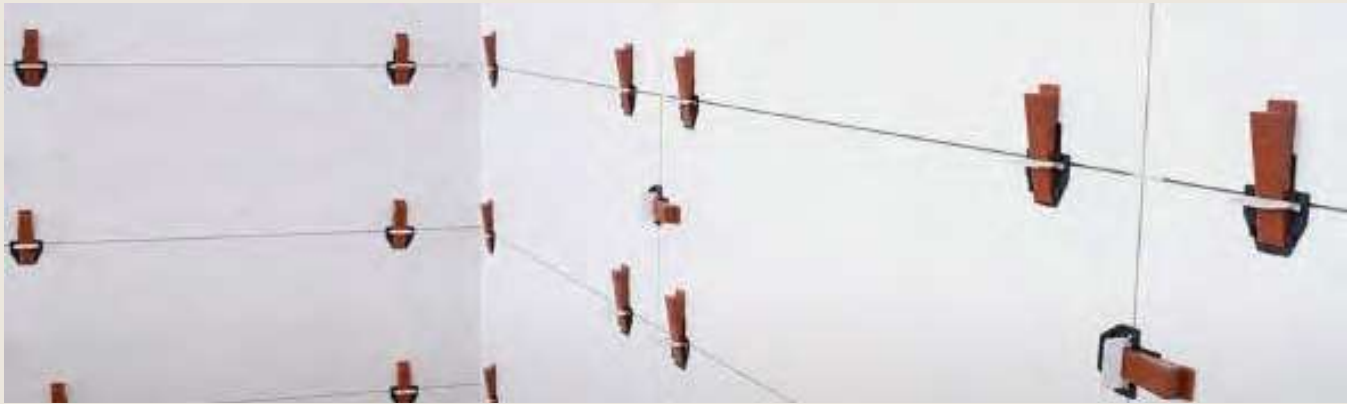
Example of using the RLS Levelling System to lay tiles on walls and floors. Exemple de pose R.S.L.
